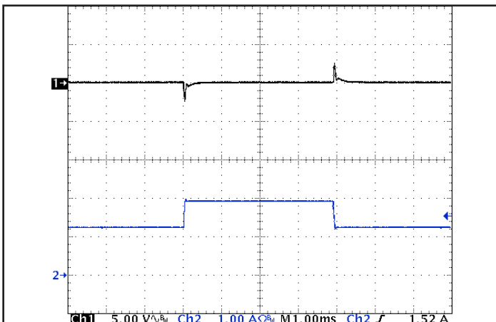
Figure 5: Output voltage response to step-change in load current (50% -75% -50% of I_{out(max)} ; dI/dt = 0.2 A/\mu s ). Load cap: 1 \mu F ceramic cap. Ch 1: V_{out} , Ch 2: I_{out} (1 A/div).
