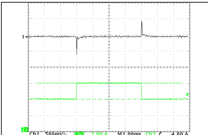
Figure 5: Output voltage response to step-change in load current (50% - 75% - 50% of I out (max); dI/dt = 0.1 A/μs). Load cap: 15 μF tantalum cap and 1 μF ceramic cap. Ch 1: V out (500 mV/div), Ch 2: I out (2 A/div). Timebase: (1 ms/div).
