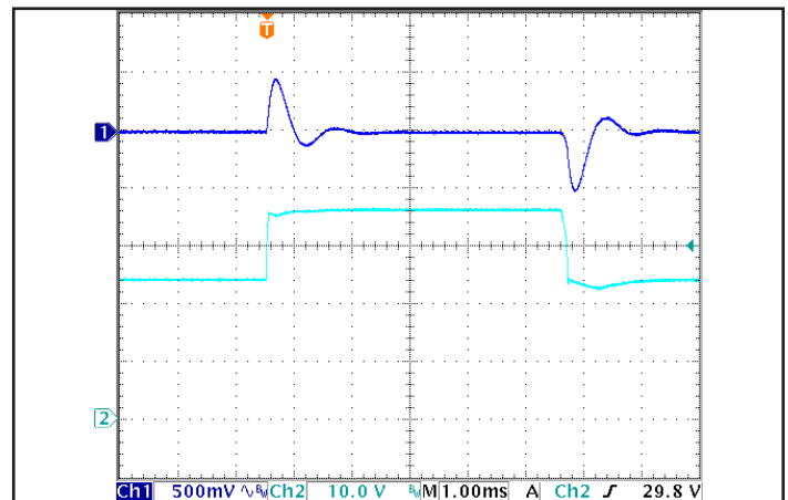
Figure 6: Output voltage response to step-change in input voltage (1000 V/ms). Load cap: 1 \mu F ceramic and 15 \mu F tantalum capacitors. Ch 1: V_{out} , Ch 2: V_{in} .
