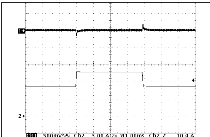
Figure 5: Output voltage response to step-change in load current (50% -75% -50% of Iout(max); dI/dt = 0.1 A/μs). Load cap: 15 μF tantalum cap and 1 μF ceramic cap. Ch 1: Vout, (500 mV/div), Ch 2: Iout (5 A/div). Timebase: (1 ms/div).
