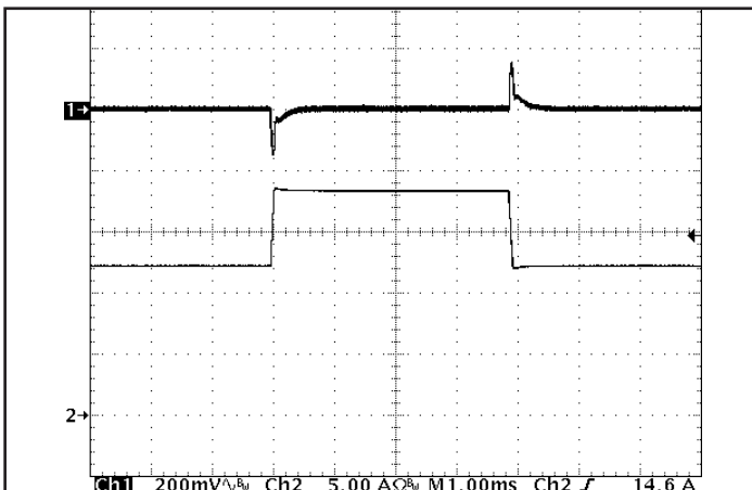
Figure 5: Output voltage response to step-change in load current (50% -75% -50% of I out (max); dI/dt = 0.1 A/μs). Load cap: 15 μF tantalum cap and 1 μF ceramic cap. Ch 1: V out , (200 mV/div), Ch 2: I out (5 A/div). Timebase: (1 ms/div).
