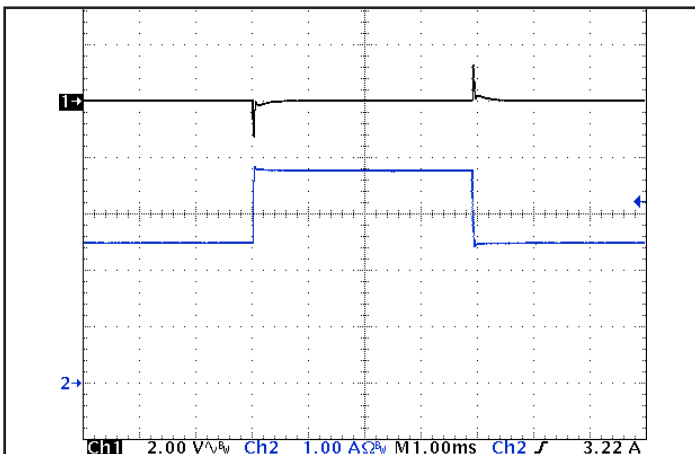
Figure 5: Output voltage response to step-change in load current (50% -75% -50% of I out (max); dI/dt = 0.8 A/μs). Load cap: 1 μF ceramic cap. Ch 1: V out , (2 V/div), Ch 2: I out (1 A/div). Timebase: (1 ms/div).
