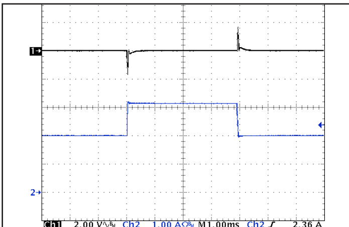
Figure 5: Output voltage response to step-change in load current (50% -75% -50% of I out (max); dI/dt = 0.5 A/μs). Load cap: 1 μF ceramic cap. Ch 1: V out , (2 V/div), Ch 2: I out (1 A/div). Timebase: (1 ms/div).
