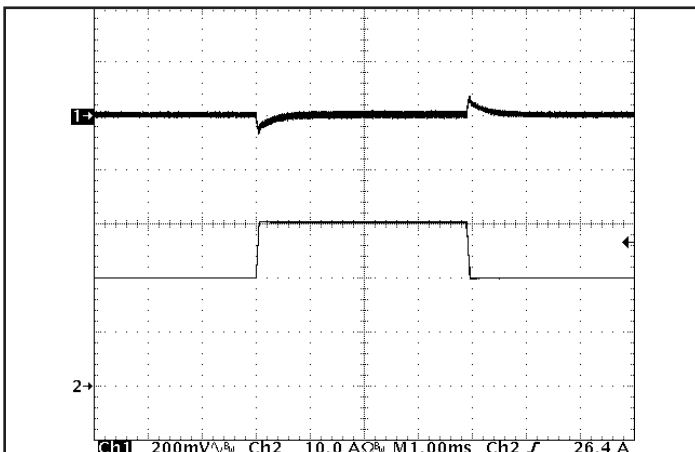
Figure 5: Output voltage response to step-change in load current (50% -75% -50% of I out (max); dI/dt = 0.2 A/μs). Load cap: 15 μF tantalum cap and 1μF ceramic cap. Ch 1: V out (200 mV/div), Ch 2: I out (10 A/div). Timebase: (1 ms/div).
